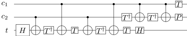
Fig. 6: Example of Toffoli gate implemented by a sequence of CNOT, T , T^\dagger , P and H gates [32]. Its TQEC implementation where T , T^\dagger , P and H gates are implemented using teleportations can be seen in Fig. 20 of [6].
