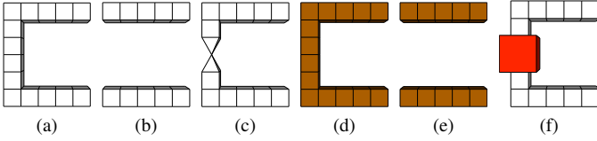
Fig. 3: Geometric components for measurement and initialization qubits. White cuboids denote primal defects and brown cuboids denote dual defects. (a) (e) Z -basis measurement and |0\rangle initialization. (b) (d) X -basis measurement and |+\rangle initialization. (c) State injection for |A\rangle or |Y\rangle initialization. (f) Generalized pin representation for primal defects where the red cube generalizes the operation of initialization or measurement [6].
