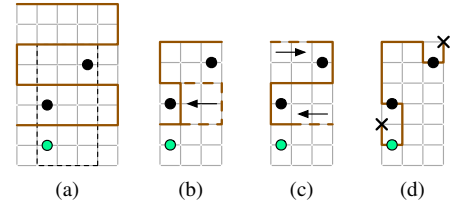
Fig. 11: Example of optimization for guidelines: (a) extract minimum bounding box that covers all qubits in the net (vertically extend by one grid for different candidates) and (b) shift vertical segments to remove redundant horizontal segments and (c) shorten dangling ending segments. (d) Example of generated routing in front face from the guideline in (b).
