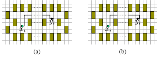
Fig. 13: Gadget to represent truth or false assignment of a variable. Example of (a) front path and (b) back path. The green rectangles denote obstacles. The source pin is marked light green and sink pin is marked black. The front path and back path are connected through their ending points.
