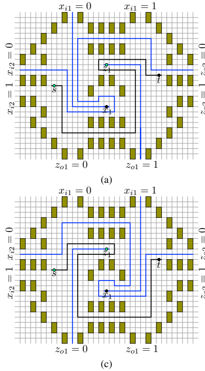
Fig. 21: Crossover with 4 cases of input: (x_{i1}, x_{i2}) = (a) 00, (b) 01, (c) 10, (d) 11. Additional inverter is required for output z_{o1} at the bottom.
