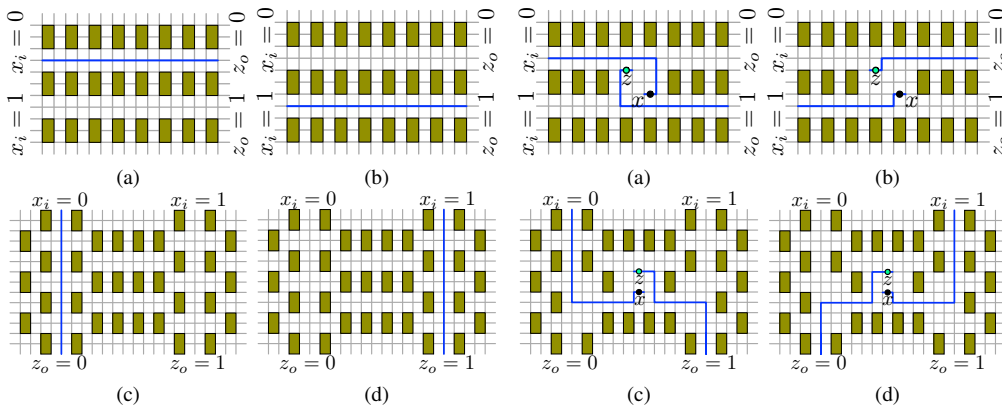
Fig. 16: Pipes with two cases of input: horizontal pipe (a) x_i = 0 , (b) x_i = 1 and vertical pipe (c) x_i = 0 , (d) x_i = 1 .
