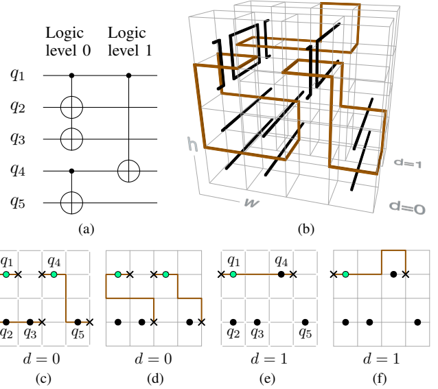
Fig. 9: (a) Example of a CNOT gate with two logic levels and (b) 3D stick diagram of its corresponding routing solution in two depth steps. Stick diagram at depth step 0: (c) front face and (d) back face. Stick diagram at depth step 1: (e) front face and (f) back face.
