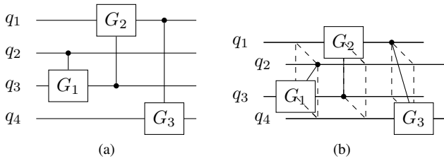
Fig. 1: Examples of (a) 1D and (b) 2D implementations of quantum circuits where qubits are arranged in 1D line or 2D space [25]. Squares labeled with “G” represent quantum gates.
