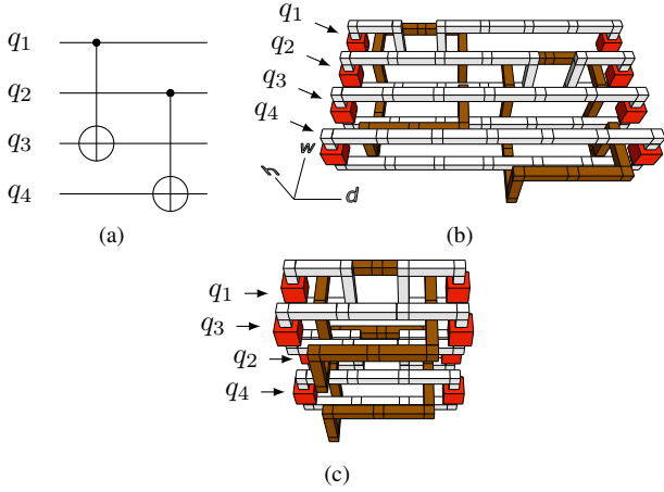
Fig. 5: Example of (a) circuit consisting of two CNOT gates with (b) 1D (single-layer) qubit arrangement with depth of 2 and (c) 2D (two-layer) qubit arrangement with depth of 1. Axis d denotes the depth axis. Axis w and h are axes for space volumes.
