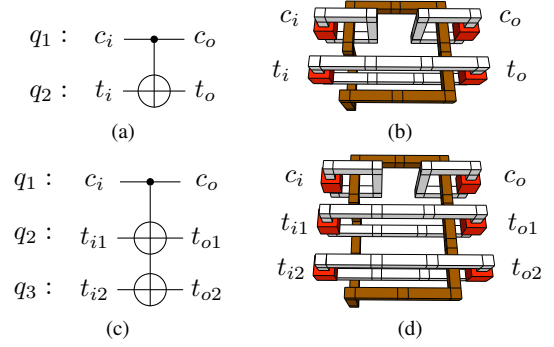
Fig. 4: (a) A CNOT gate with q_1 as control qubit and q_2 as target qubit. (b) The primal-primal implementation of CNOT gate where dual defects (brown) braid around primal defects (white) and red cubes represent inputs and outputs [8]. (c) A multiple-target CNOT gate with q_1 as control qubit and q_2 and q_3 as target qubits. (d) Geometric description of the multiple-target CNOT gate.
