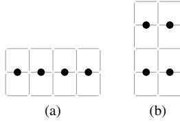
Fig. 8: (a) Example of single-layer qubit arrangement like that in Fig. 5(b) (view from left). (b) Two-layer qubit arrangement like that in Fig. 5(c).
