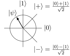
Fig. 2: Quantum state and different bases ( |0\rangle and |1\rangle for Z -basis and |+\rangle and |-\rangle for X -basis).
