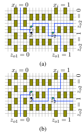
Fig. 18: Junction with two cases of input: (a) x_i = 0 (b) x_i = 1 . Additional inverter is required for output z_{o1} at the bottom.
