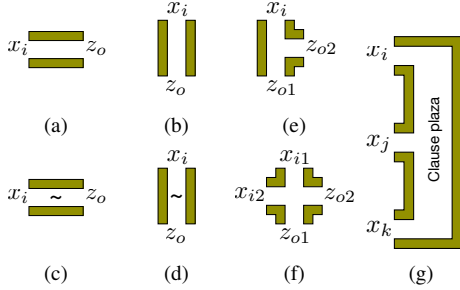
Fig. 14: Some symbols of gadgets. (a) Horizontal and (b) vertical pipe ( z_o = x_i ). (c) Horizontal and (d) vertical inverter ( z_o = \bar{x}_i ). (e) Junction ( z_{o1} = z_{o2} = x_i ). (f) Crossover ( z_{o1} = x_{i1}, z_{o2} = x_{i2} ). (g) Clause plaza where there is feasible routing solutions iff the clause has truth assignment.
