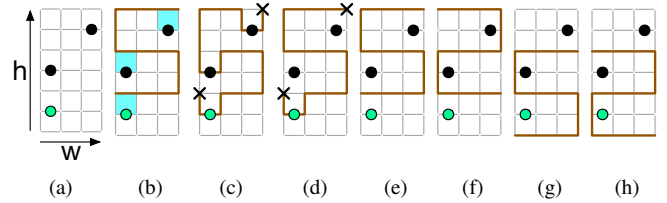
Fig. 10: (a) Example of net where control qubit is marked by green dot and target qubits are marked by black dots and (b) a guideline for generating routing solution and (c) generated front face and (d) back face. Four possible guidelines for a net are shown in (e) (f) (g) (h).
