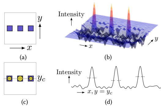
Figure 2: (a) Design target of 3 contacts and (b) the light intensity plot of aerial image. Assume that RETs such as SRAF and OPC have been already applied to the contacts before optical simulation. (c) A dotted line horizontally crosses the centers at y = y_c and the circles denote the contours of printed patterns. (d) Light intensity profiling along the dotted line at y = y_c extracted from the aerial image and different slicing thresholds for each contact.
