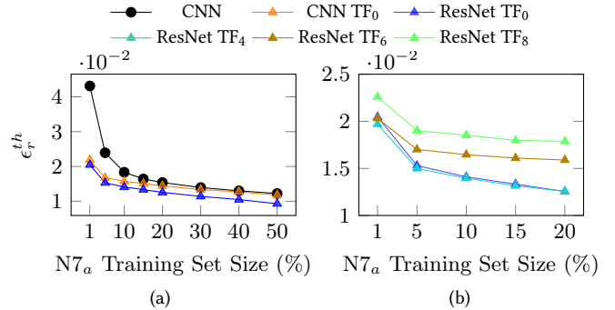
Figure 13: Testing accuracy of transfer learning from N10 to N7_a . (a) Comparison between CNN and transfer learning. (b) Comparison between transfer learning schemes where different numbers of layers are fixed.
