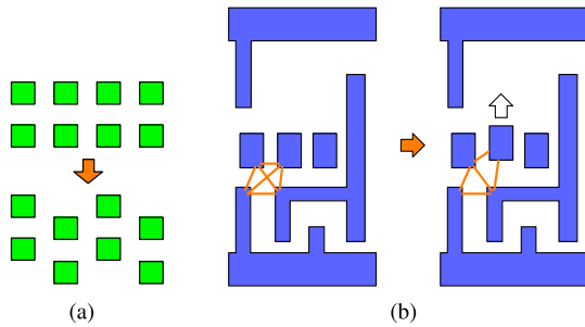
Fig. 3. Native conflict removal for (a) contact layer and (b) M1 layer.
