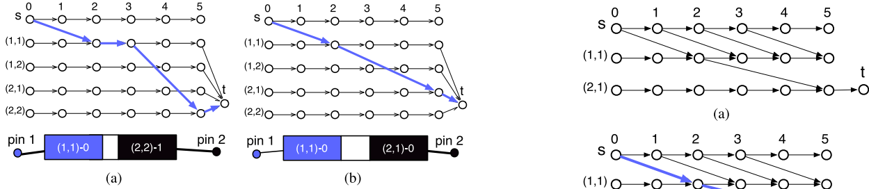
Fig. 10. Shortest path solutions on the graph model with (a) 1 stitch and (b) 0 stitch.
