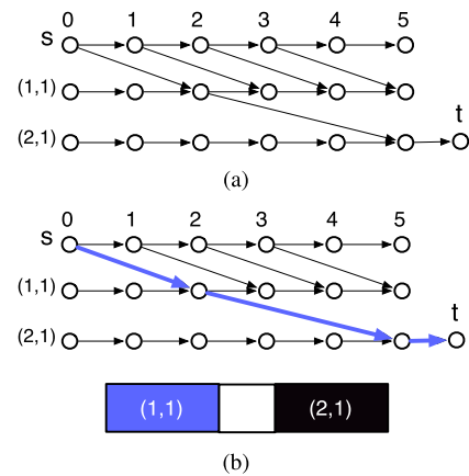
Fig. 12. (a) Second stage to solve detailed placement. (b) One shortest path solution corresponds to a cell placement.
